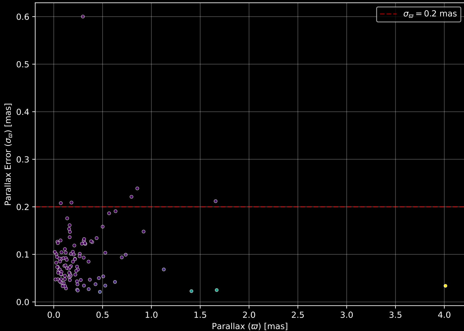
APOGEE DR17 Field: [356-03-O] Parallax Quality (n= 109)
